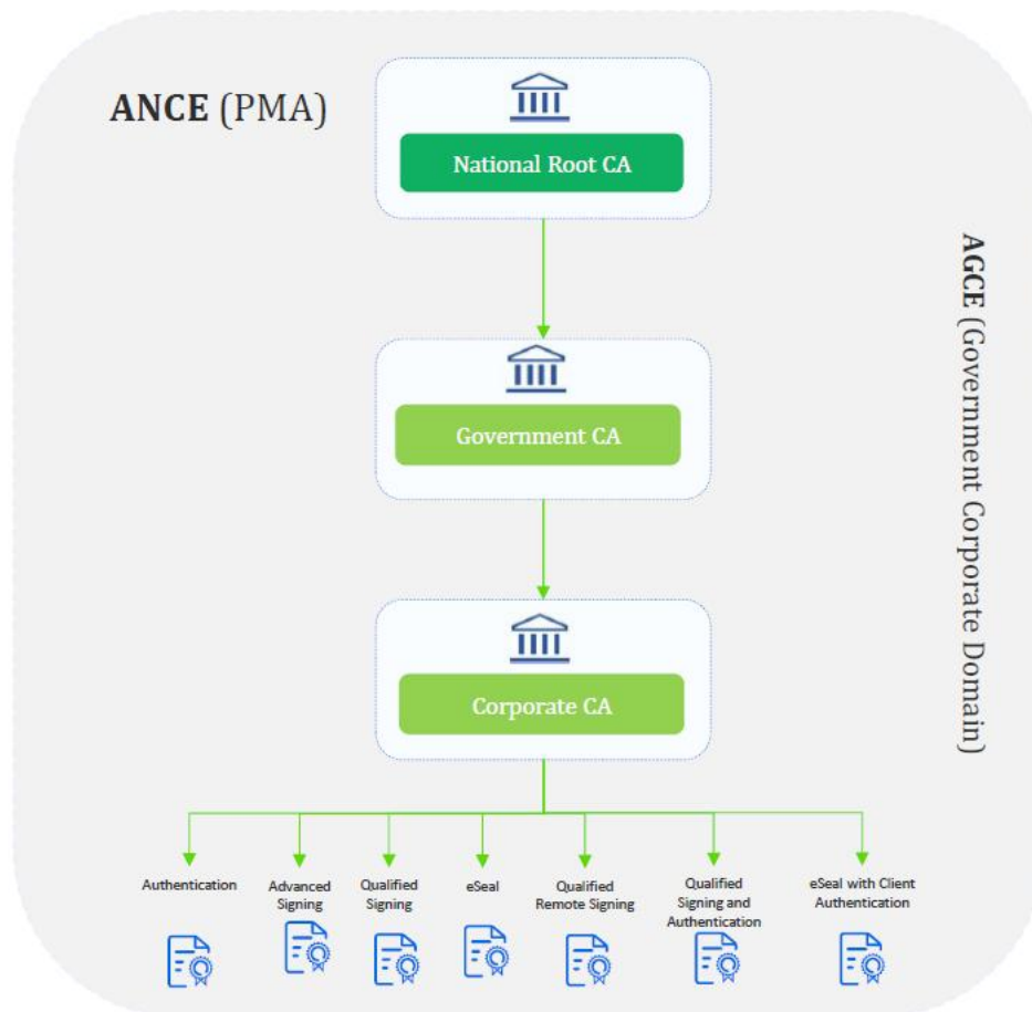
Figure 1: The Government PKI Corporate Domain
