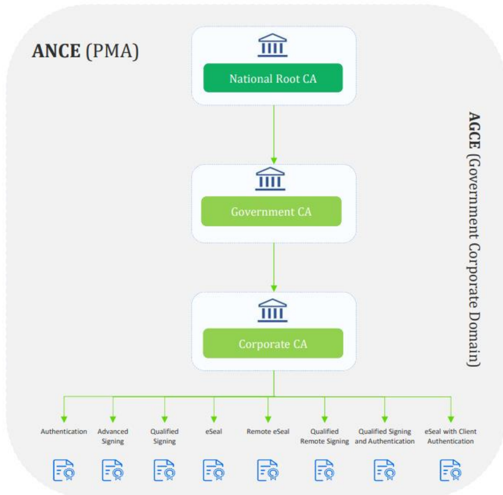
Figure 1: The Government PKI Corporate Domain
